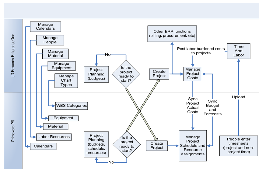
Figure 1. Oracle PPM Integration Pack Process Flow
